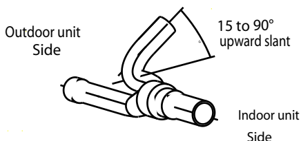
In case of horizontal position
